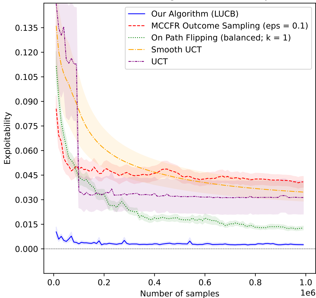
Leduc Poker, Best Algorithms (new), Player x
